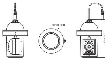
Camera: GP-330
