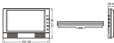
Receiver: GP-716
